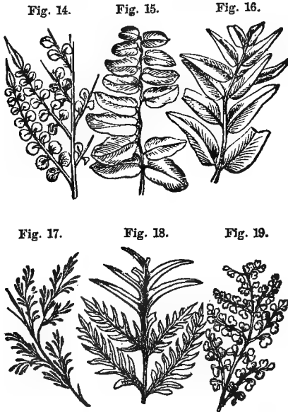
FERNS OF THE COAL MEASURES.*
